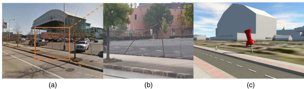
Fig. 5. Example of a vulnerable object recognized through participatory sensing and the localization: (a) an image from Google Earth (without vulnerable condition) (Image Capture: Dec 2018 ©2019 Google); (b) an example of crowdsourced visual data involving a vulnerable object (during our data collection); and (c) crowdsourced visual sensing-driven localization in a city model.
