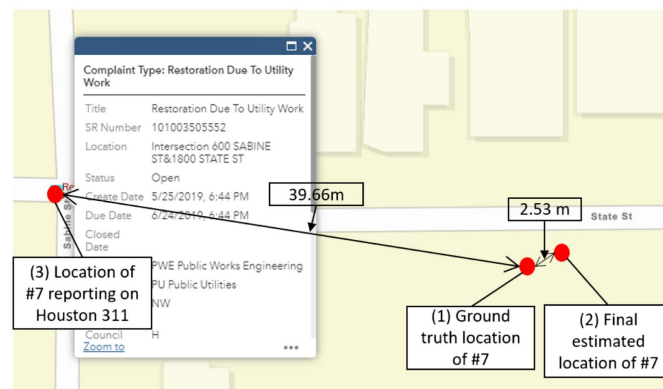
Fig. 8. Comparison of localization errors between the proposed method and Houston 311 service map for object #7: (1) ground truth location of the vulnerable object; (2) final estimated location of the object through the proposed method; and (3) mapping location of the object through Houston 311 service map.
