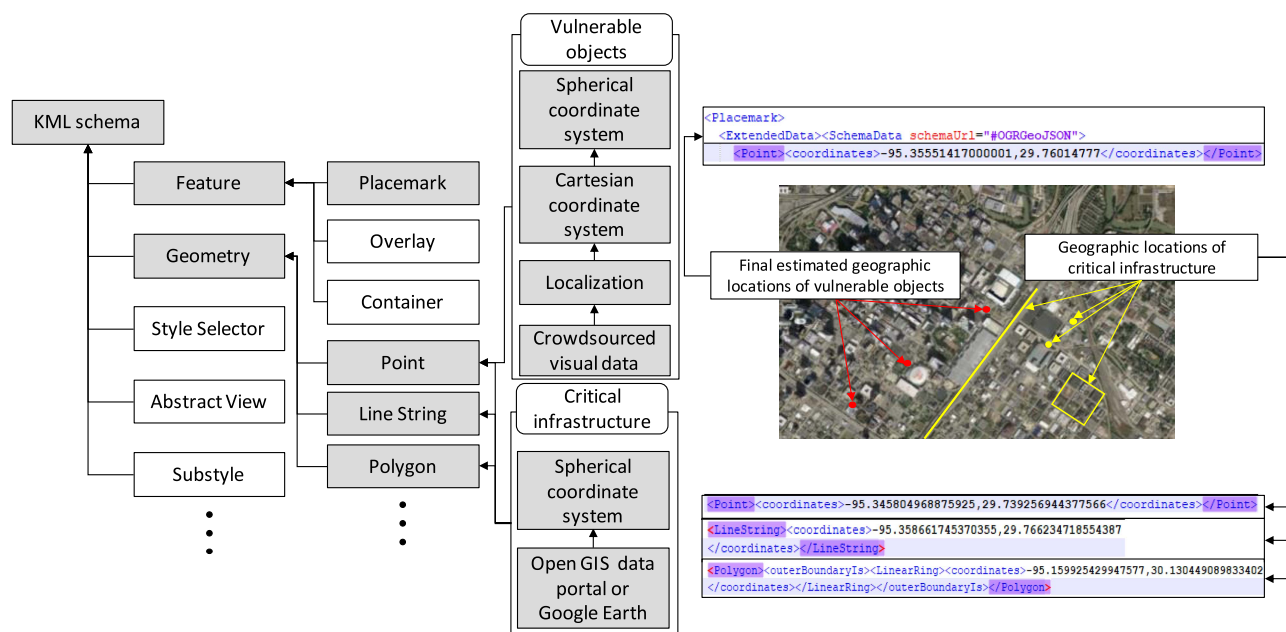
Fig. 4. Logical structure of the elements in the KML schema and an example of mapping critical infrastructure and vulnerable objects. (Imagery ©2019 Google, Map data ©2019.)
