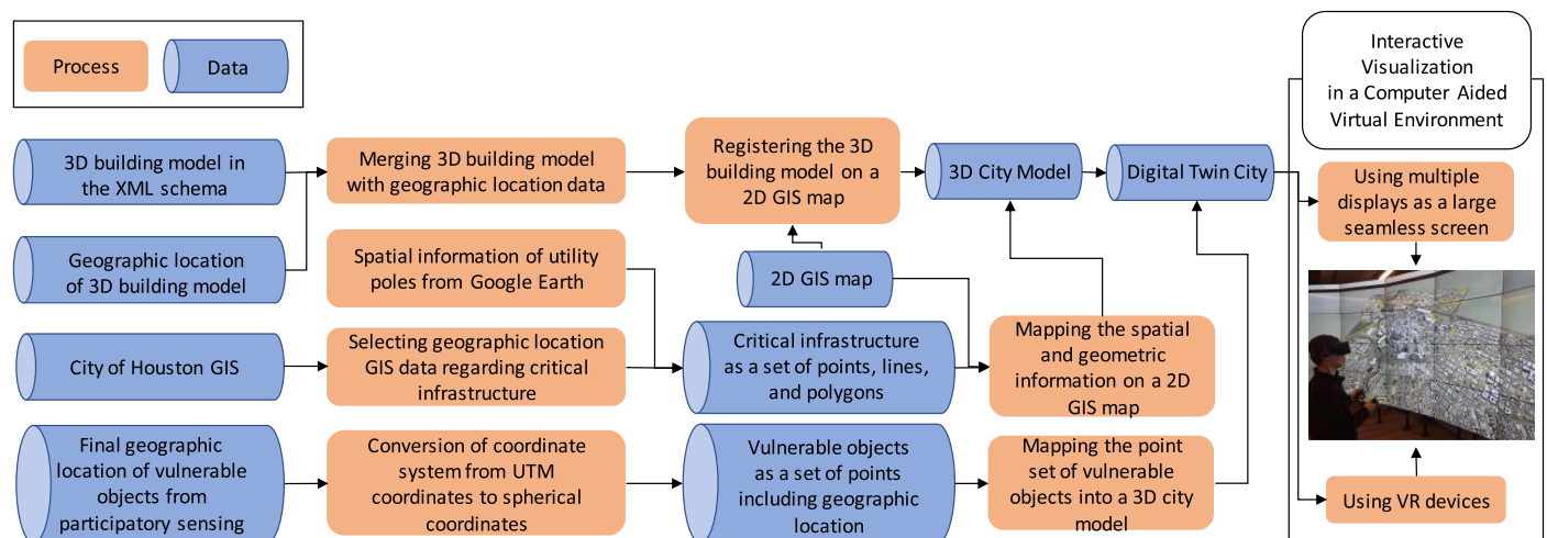
Fig. 3. Overview of the data and process toward an updated 3D virtual model of Houston. XML, extensible markup language.
